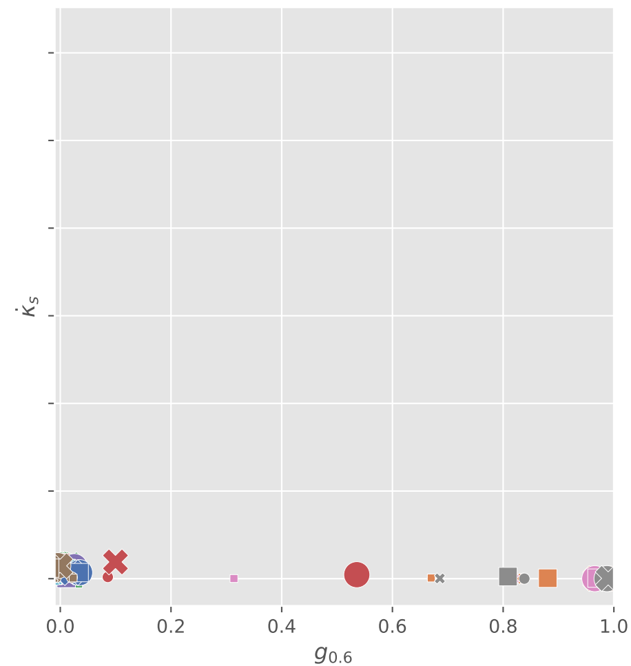
K = \text{abs}
