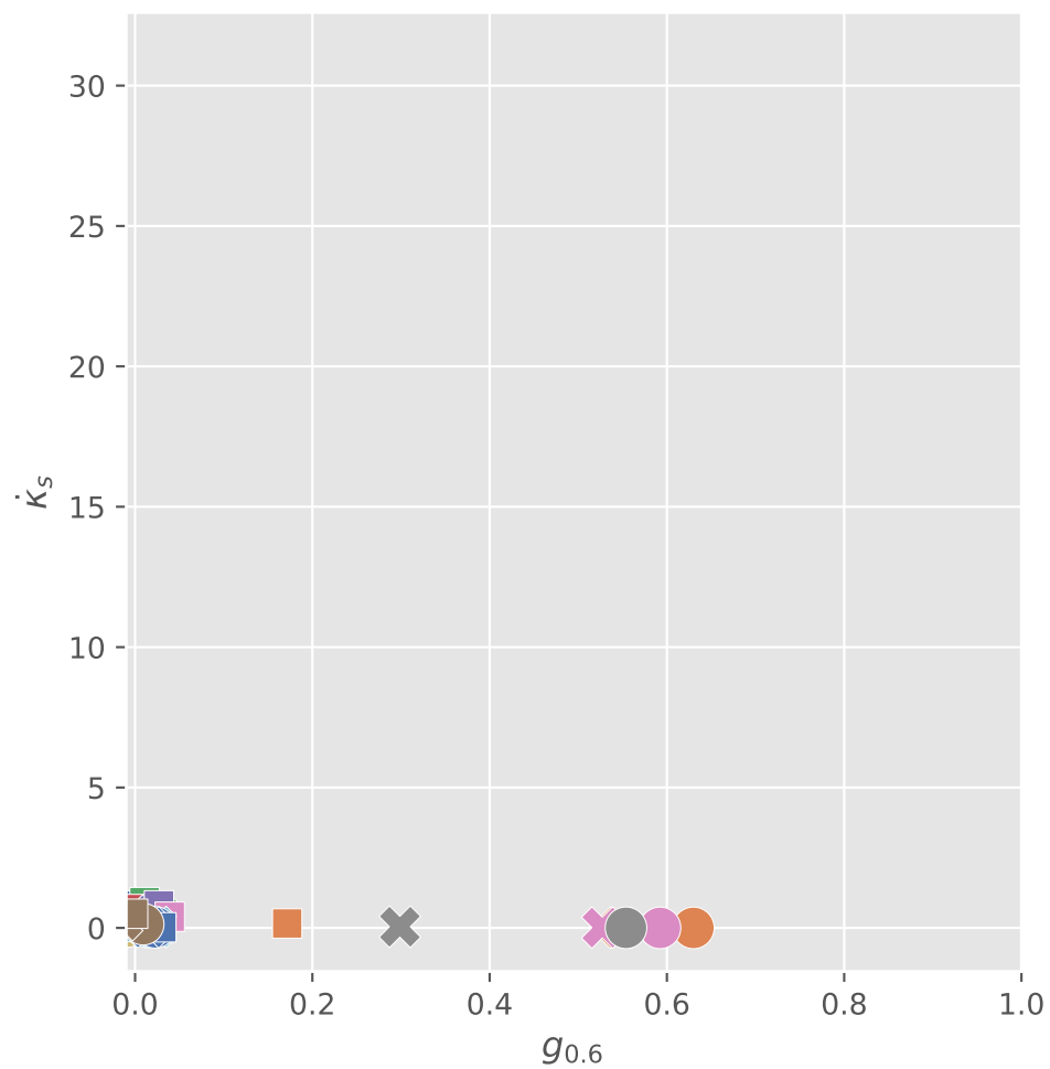
K = \text{product}
